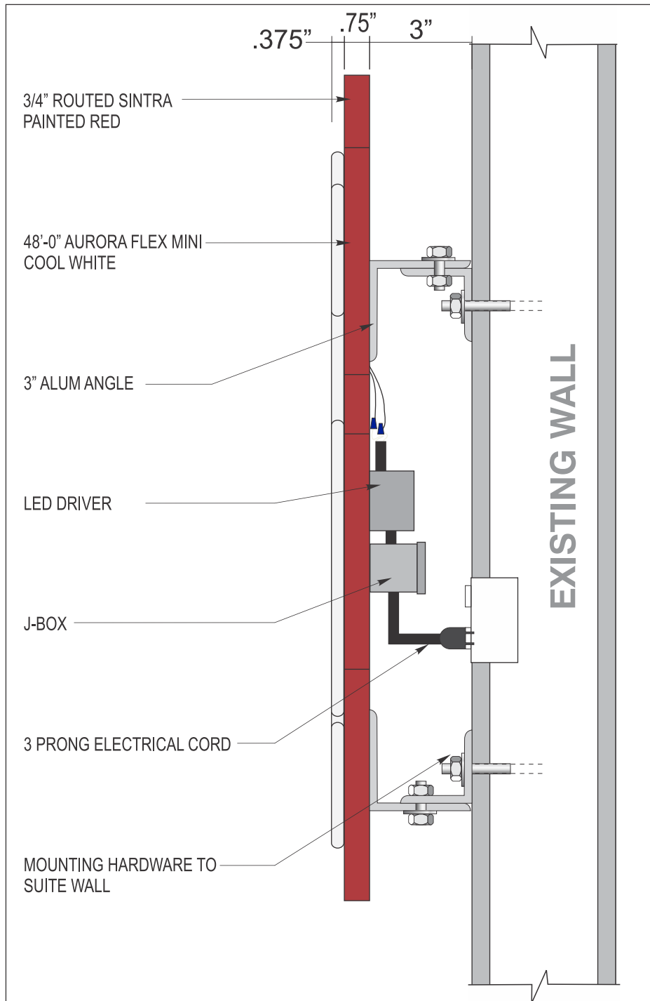
SECTION @ ROUTED SINTRA/LED LIT SCALE: X3
